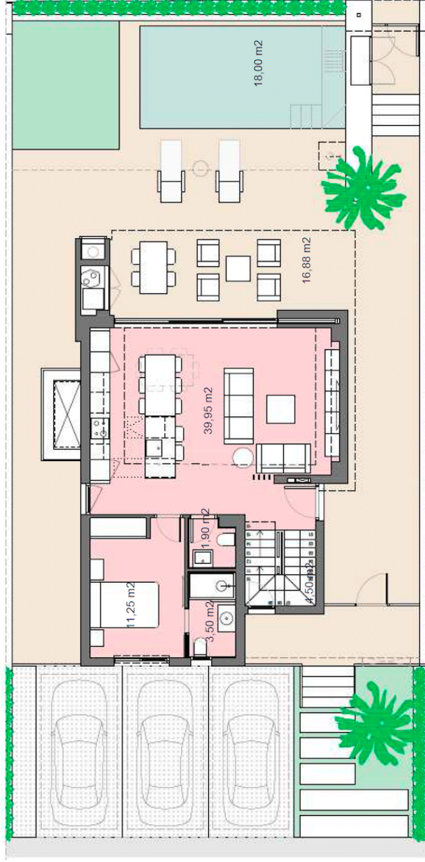
GROUND FLOOR
